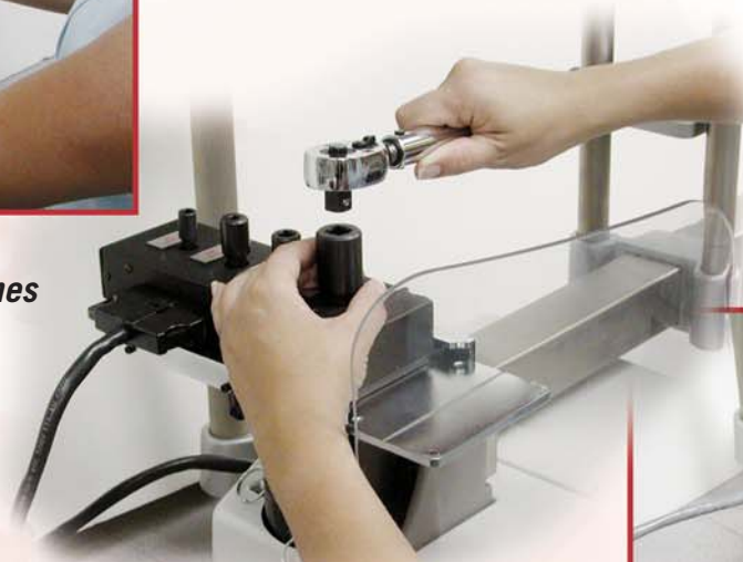
4 in 1 Transducer with Adapter Kit
